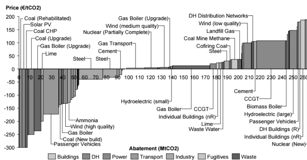
Figure 11: MACC for Status Quo Policy Scenario (2030)
