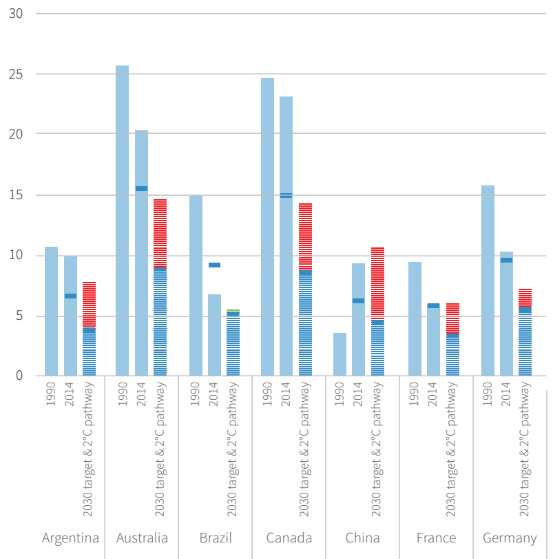
Emissions per capita (tCO 2 -eq/capita, including LULUCF), historic values,
