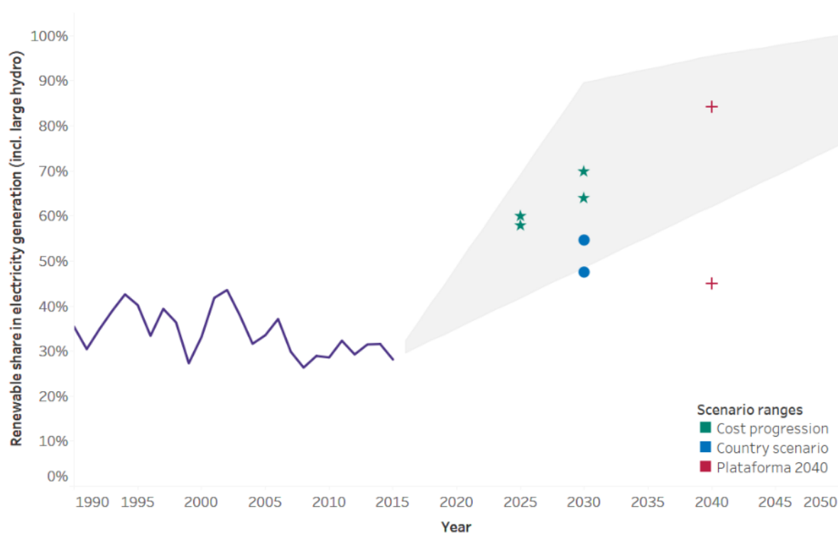
Figure 8 Renewable electricity generation shares compared to a Paris compatible range. The marks correspond to the minimum and maximum values of renewable shares in the respective analyses. See Box A for more information on the scenarios.
