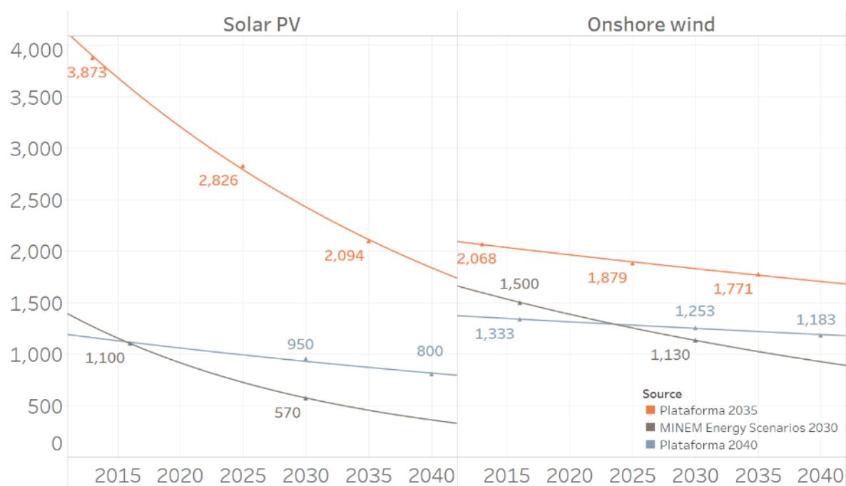
Figure 3 Investment costs projections for onshore wind and solar PV. The orange cost curve represents pre-NDC cost expectations and the others (gray and blue) post-NDC cost expectations.
