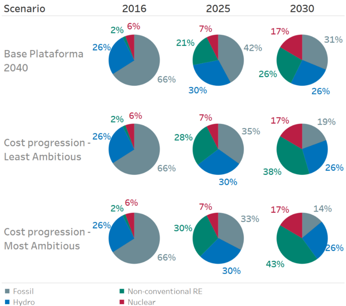
Figure 7 Evolution of power generation shares in Argentina under the base case scenario and least and most ambitious cost progression scenarios.
