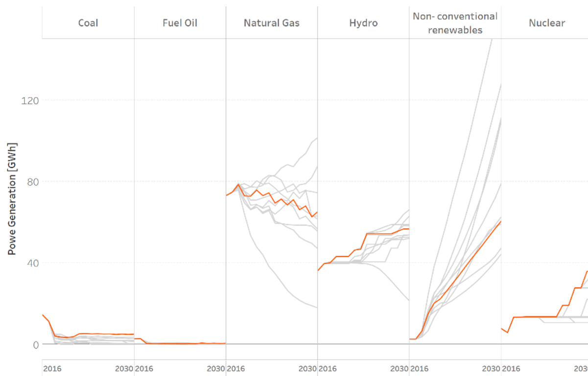
Figure 2 Power generation from Plataforma Escenarios 2040 ; base case scenario highlighted in orange.
