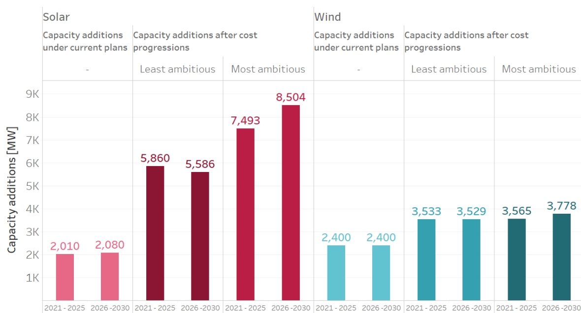
Figure 6 Capacity additions within the specified timeframes for solar PV and onshore wind before and after cost progression considerations.
