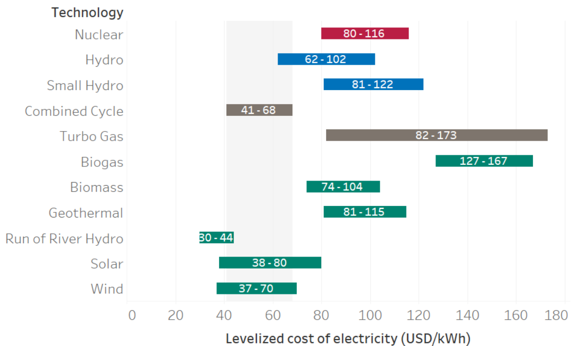
Figure 5 Levelized cost of electricity per technology. The colours match Argentina's definition of non-conventional renewables (green), fossil fuels (grey), hydro (blue) and nuclear (red). The ranges include broader costs such as those covering the transportation of natural gas for fossil fuel technologies or grid expansion, included in the range of solar PV and wind.
