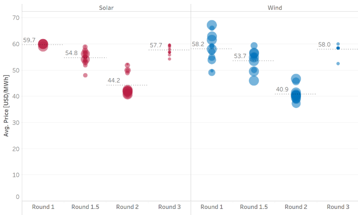
Figure 4 Average prices per MWh for wind and solar power generation contracted under the RenovAr programme. Each bubble represents a distinct project, the bubbles' size reflects the installed capacity.
