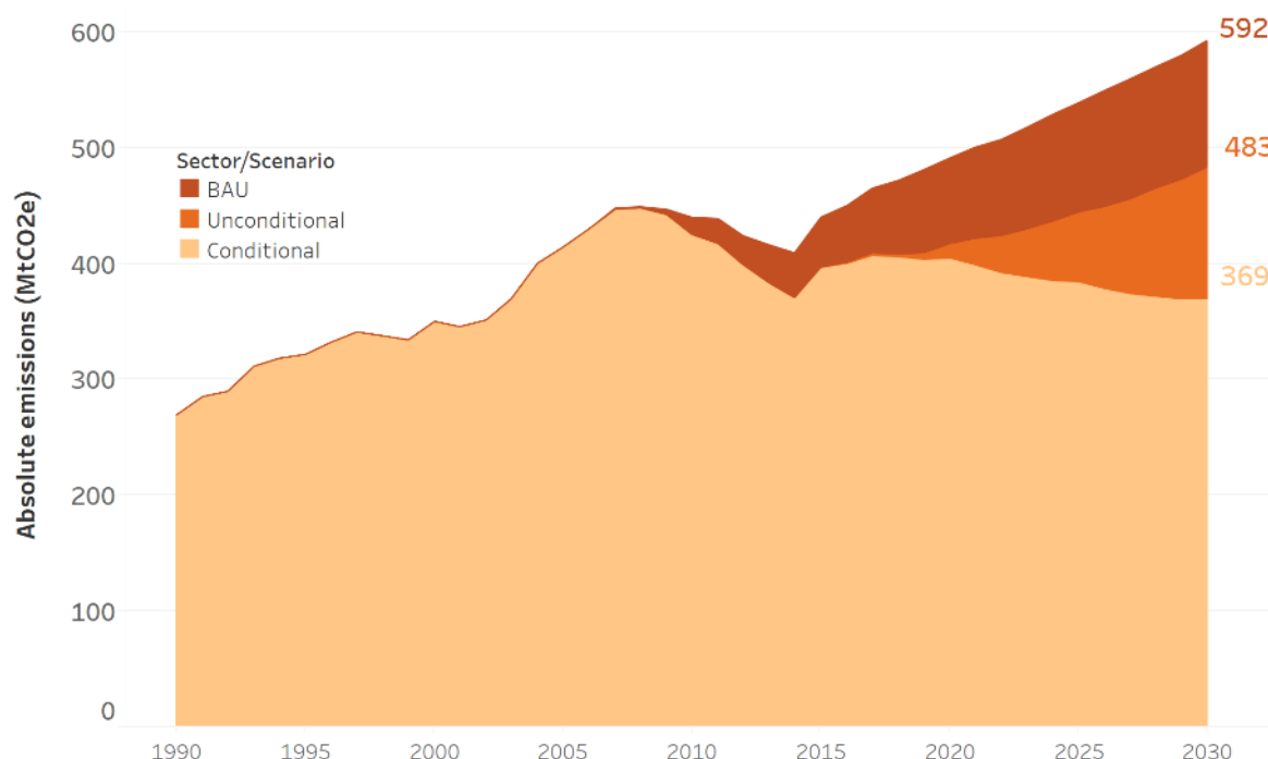
Figure 1 Argentina's GHG emissions projections according to the NDC.
